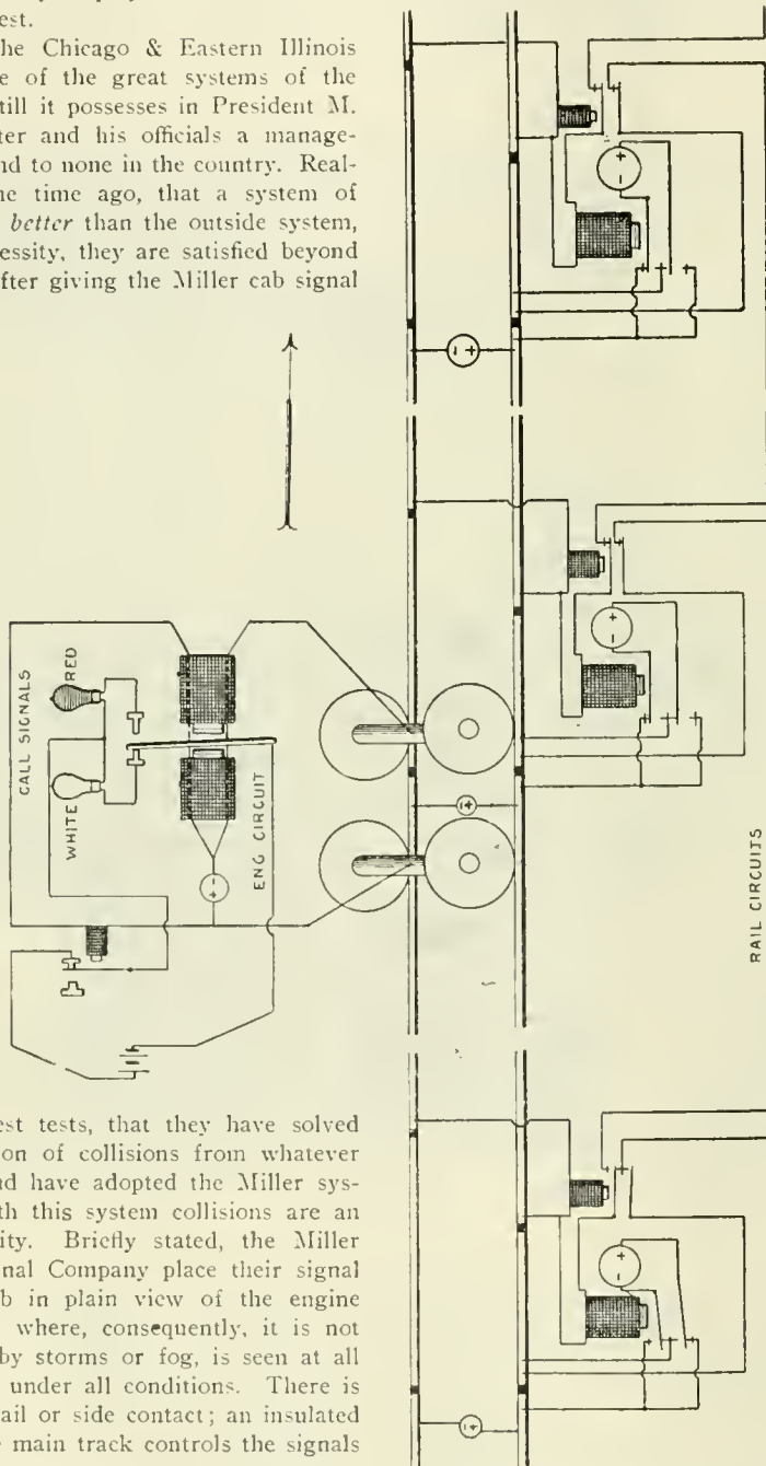
NEW SIGNALLING SYSTEM OF THE CHICAGO & EASTERN ILLINOIS RAILROAD.
